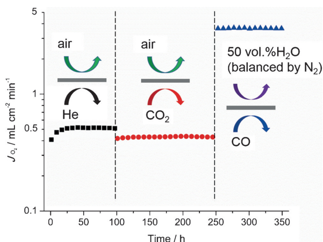
Figure 3. Long-term oxygen permeation rates ( J_{\text{O}_2} ) through the non-infiltrated SDC–SSAF symmetrical dual-phase membrane. Conditions: air = 100 mL min −1 or H 2 O = 50 mL min −1 (balanced by 50 mL min −1 N 2 ) as the feed gas; He = 50 mL min −1 or CO 2 = 30 mL min −1 or CO = 30 mL min −1 as the sweep gas, respectively. 1 mL min −1 Ne as the internal standard gas. Temperature = 950 °C.
